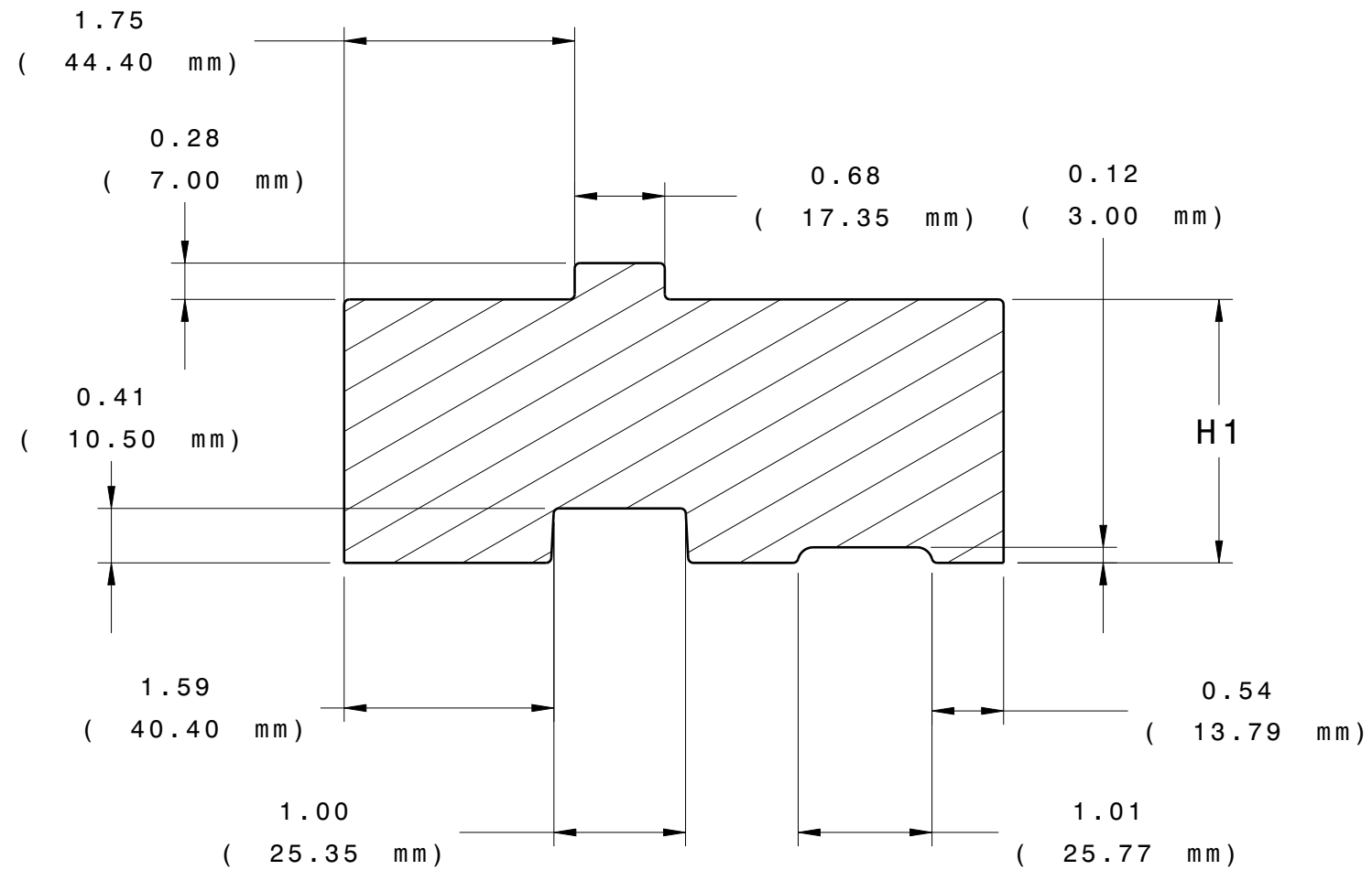
Section Mating Components
